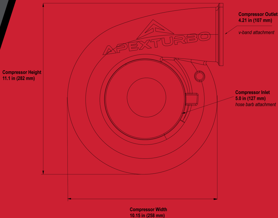
APX 500 Compressor Housing
